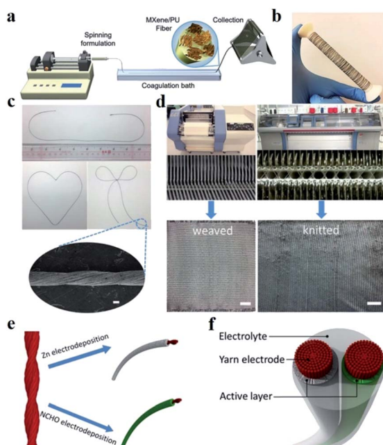
Fig. 7 (a) Schematic illustration of the wet-spinning process of the MXene/PU fiber. (b) Digital photograph of fabricated MXene/PU fiber. Reproduced with permission. 120 Copyright 2020, Wiley-VCH. (c) Flexibility demonstration and SEM image of the yarn. (d) Demonstration of weavability and knittability. (e) Schematics of yarns electrodeposited with Zn and NCHO and (f) solid-state yarn battery. Reproduced with permission. 121 Copyright 2017, American Chemical Society.
