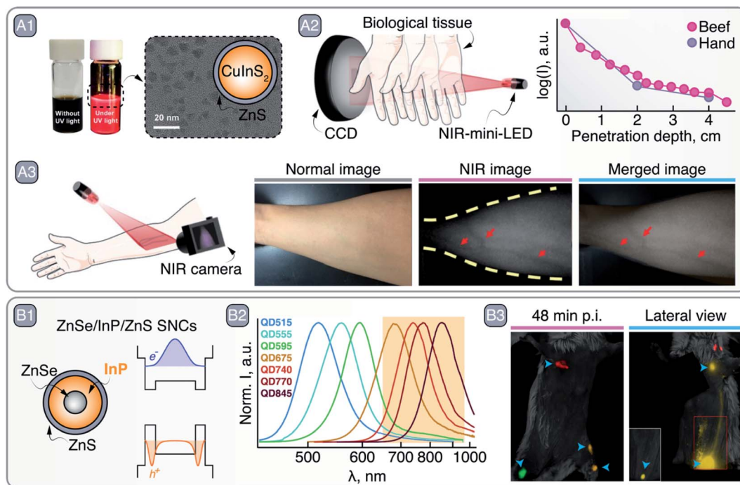
Fig. 5 A – \text{CuInS}_2/\text{ZnS} SNCs as NIR-emitting mini-LEDs: A1 – bright field and NIR PL photographs of \text{CuInS}_2/\text{ZnS} SNC dispersions, as well as their TEM image and graphical representation. A2 – NIR PL of \text{CuInS}_2/\text{ZnS} SNCs penetration through tissues. A3 – vein imaging with \text{CuInS}_2/\text{ZnS} SNCs mini-LED. Adapted with permission of Royal Society of Chemistry, from ref. 52; permission conveyed through Copyright Clearance Center, Inc. B – \text{ZnSe}/\text{InP}/\text{ZnS} SNCs as NIR imaging agents: B1 – schematic of the core/shell/shell \text{ZnSe}/\text{InP}/\text{ZnS} SNCs and their bandgap alignments with corresponding electron and hole wave functions. B2 – change in the PL spectrum peak position of \text{ZnSe}/\text{InP}/\text{ZnS} SNCs as a function of InP deposition. B3 – left inguinal LN, axillary LN, and right inguinal LN and popliteal LN multiplexed imaging with different \text{ZnSe}/\text{InP}/\text{ZnS} SNCs 48 min post injection (p.i.). Lateral view, 1 h p.i., shows SNCs lymphatic drainage from the inguinal LN to the axillary LN; inset image with higher thresholding shows the contrast localized in the inguinal LN without image saturation. Adapted with permission from ref. 55. Copyright 2021 American Chemical Society.
