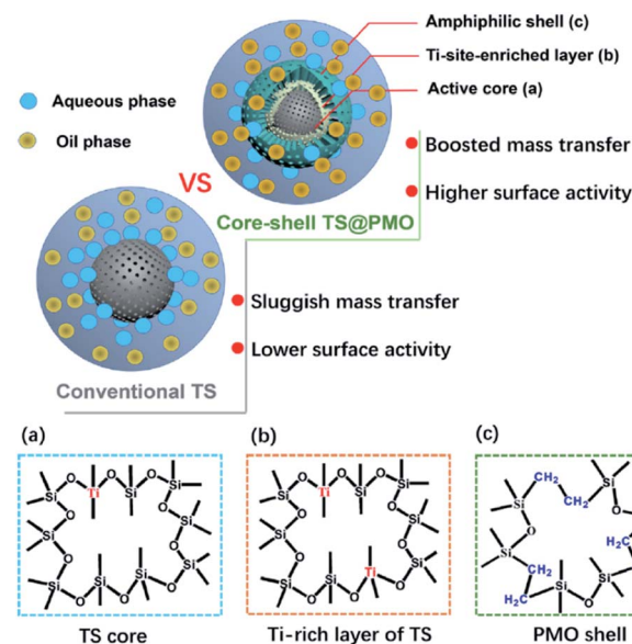
Fig. 4 Illustration of TS and TS@PMO showing the merits of material design with an amphoteric shell and surface-Ti-enriched core (a), (b), and (c) indicate the skeleton structure of the TS core and PMO shell; note: (b) is the outer layer of (a). 68 Reproduced with permission. 68 Copyright 2021, Elsevier.
