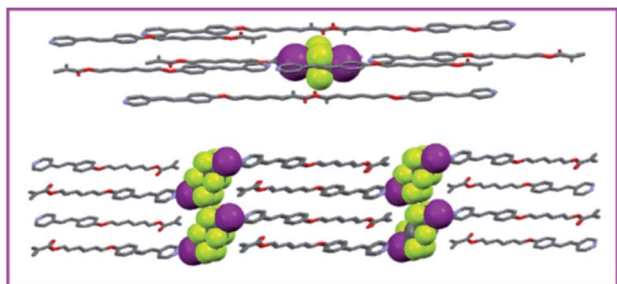
Fig. 4 Partial view of the crystal packing of the XB-based LC in ref. 59. Adapted with permission from ref. 59. Copyright 2017, Elsevier.
