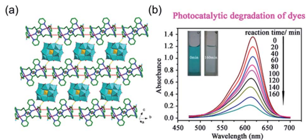
Fig. 3 (a) Crystal structure of [Ag_4(H_2O)(L)_3(SiW_{12}O_{40})] ( L = 1,4-bis(3-(2-pyridyl)pyrazol)butane); (b) UV-vis absorption and photocatalytic degradation of MG. Reproduced with permission from ref. 61. Copyright © 2016 Elsevier.
