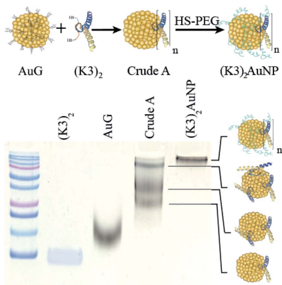
Fig. 3 PAGE analysis of reaction products obtained by the reaction of AuG with 3 molar equivalent of the thiolated K3 dimer (Crude A) and then thiolated PEG 2000 Da ( (\text{K}3)_2\text{AuNP} ).
