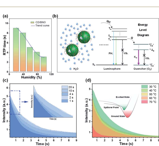
Fig. 5 (a) PH time in response to humidity. (b) The influence mechanism of humidity on PH time (Q: quenching; ^1\Delta_g : the first excited state; ^1\Sigma_g^+ : the second excited state; ^3\Sigma_g^- : triplet ground state; K_O : singlet oxygen). (c) The response of PH time to the duration of excitation with the light source. (d) The response of PH time to external temperature.
