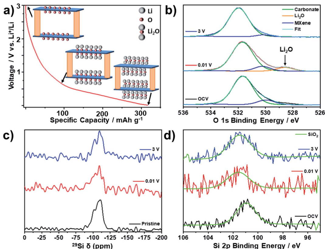
Fig. 6 Ex situ MAS SS-NMR spectra (16.4 T, 30 kHz MAS) and XPS spectra of \text{Mo}_2\text{TiC}_2 -Si-400 at selected states-of-charge. (a) Schematic illustrating the lithiation mechanism for oxygen-terminated \text{Mo}_2\text{TiC}_2 , with the MXene sheets shown in blue and the pillars in orange. (b) Ex situ O 1s XPS spectra. (c) Ex situ ^{29}\text{Si} MAS SS-NMR spectra. (d) Ex situ Si 2p XPS spectra.
