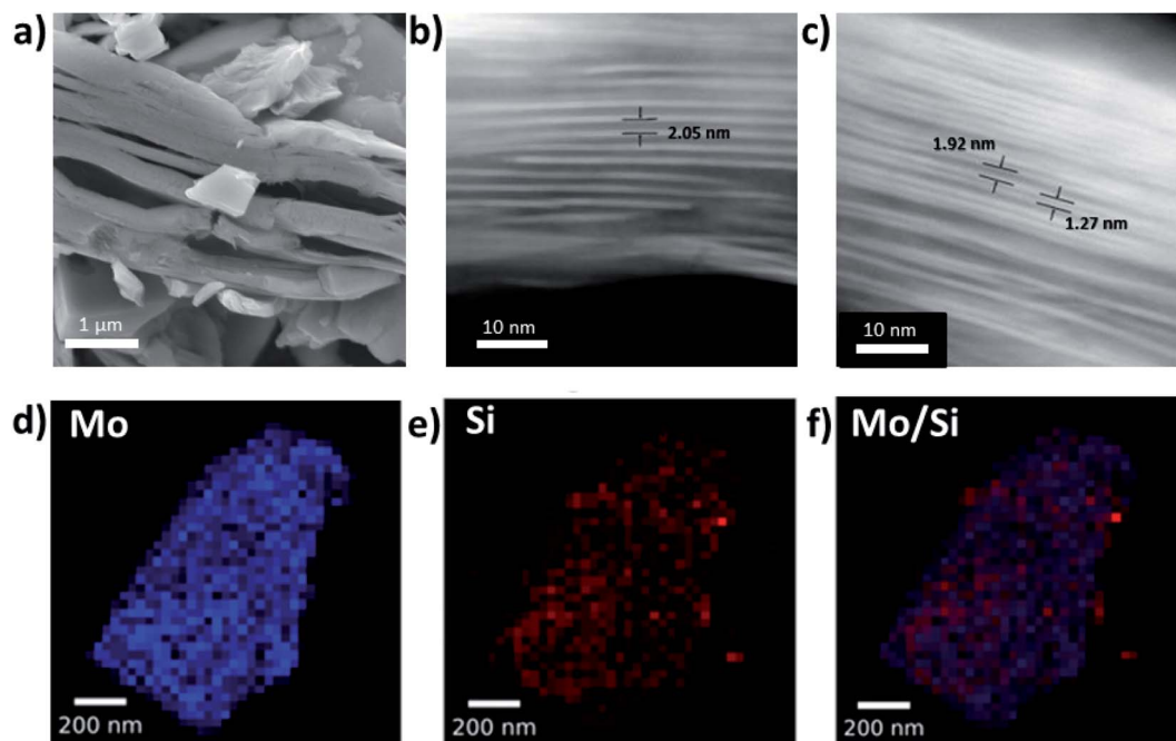
Fig. 3 (a) SEM micrograph of \text{Mo}_2\text{TiC}_2\text{-Si-400} MXene after calcination at 400^\circ\text{C} for 5 h under flowing argon. (b and c) HAADF-STEM micrographs of (b) Si intercalated MXene, \text{Mo}_2\text{TiC}_2\text{-Si} , and (c) Si-pillared and calcined MXene, \text{Mo}_2\text{TiC}_2\text{-Si-400} . (d and f) STEM-EDS maps of Si-pillared MXene, \text{Mo}_2\text{TiC}_2\text{-Si-400} showing the Mo (d) and Si (e) distribution in the pillared MXene, with the overlay shown in (f).
