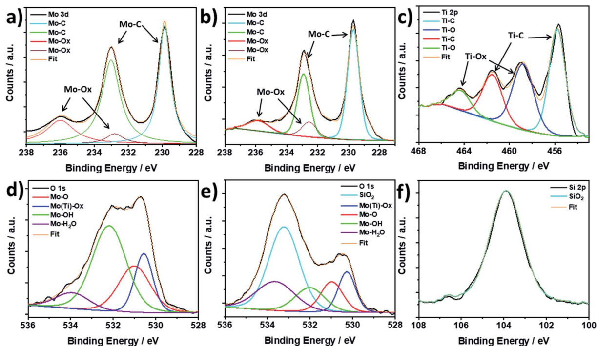
Fig. 4 Mo 3d XPS spectra for (a) non-pillared \text{Mo}_2\text{TiC}_2 and (b) \text{Mo}_2\text{TiC}_2\text{-Si-400} after calcination at 400^\circ\text{C} , \text{Mo}_2\text{TiC}_2\text{-Si-400} . (c) Ti 2p XPS spectra of \text{Mo}_2\text{TiC}_2\text{-Si-400} . (d) O 1s spectra of non-pillared \text{Mo}_2\text{TiC}_2 . (e) O 1s spectra of the pillared MXene \text{Mo}_2\text{TiC}_2\text{-Si-400} . (f) Si 2p spectra of the pillared MXene \text{Mo}_2\text{TiC}_2\text{-Si-400} .
