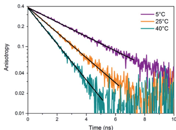
Fig. 18 Anisotropy decays of a NIR Ag N -DNA in 10 mM NH 4 OAc aqueous solution at 5 °C, 25 °C, and 40 °C. Data was fitted assuming a single rotational correlation time. 176 Adapted from Bogh, et al. , (ref. 176) with permission from the Institute of Physics.
