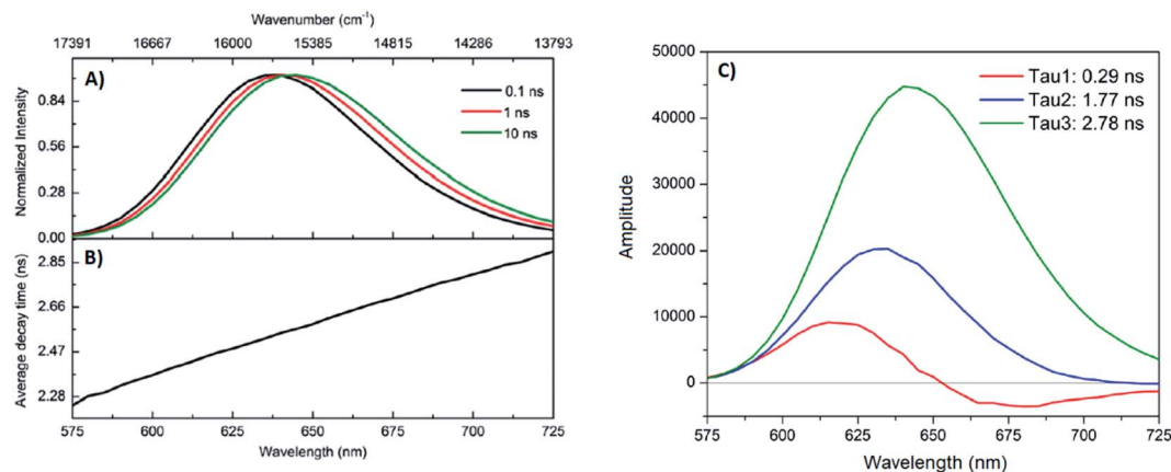
Fig. 17 (A) TRES, (B) average decay time as a function of emission wavelength, and (C) DAS of red emissive Ag N -DNAs at 25 °C, excited at 561 nm. The gray line in (C) indicates the zero line. In order to construct TRES and DAS, the intensity decays were acquired from 575 nm to 725 nm, in steps of 5 nm. The three decay time values were globally linked in the fit. 185 Adapted from Cerretani, et al. , (ref. 185) with permission from the Royal Society of Chemistry.
