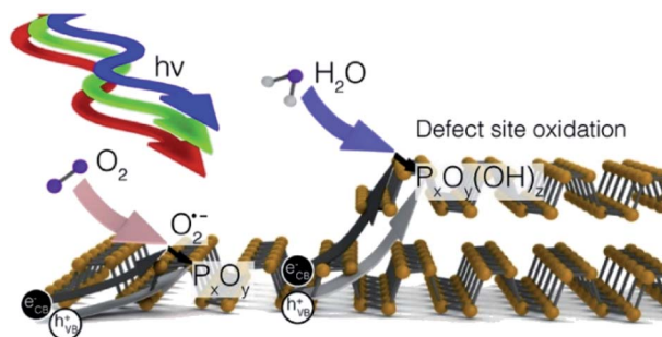
Fig. 3 Degradation process of black phosphorus. 55 (Copyright 2017 J. Am. Chem. Soc. )
