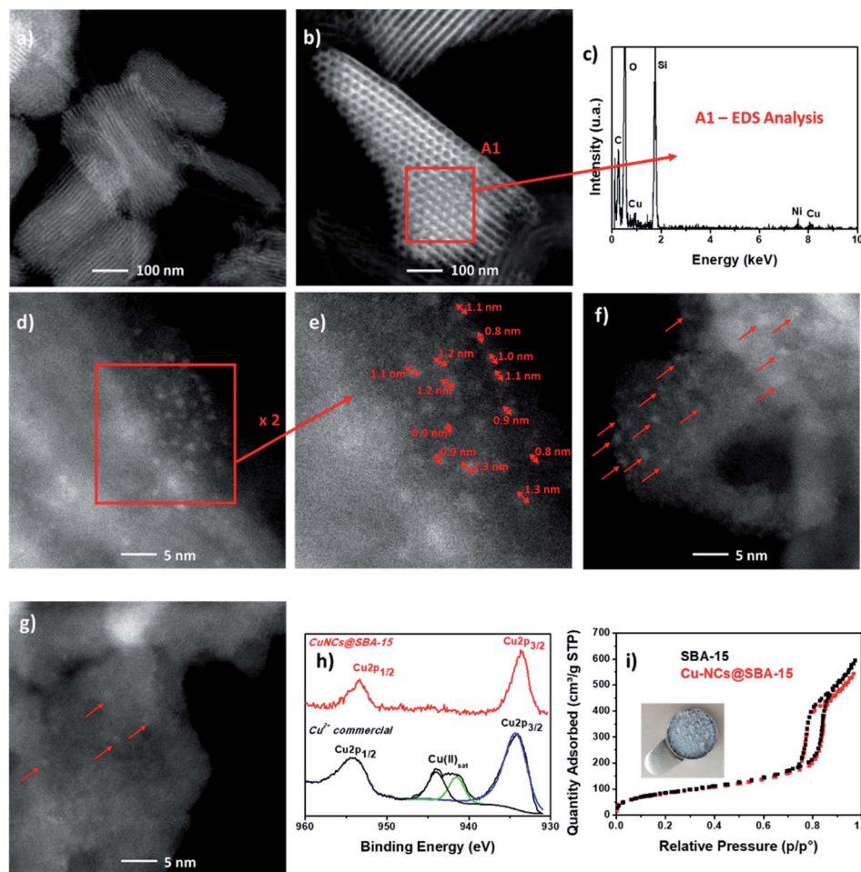
Fig. 2 (a and b) HAADF-STEM analysis of Cu-NCs@SBA-15 with the selection of an area of 4 \mu\text{m}^2 and (c) its relative EDS analysis. (d–g) HAADF-STEM analysis of Cu-NCs smaller than 2 nm. (h) Cu 2p XPS core level of Cu-NCs@SBA-15 in red and Cu(II) pattern in black showing the characteristic satellite peaks. (i) \text{N}_2 adsorption curve for the mesoporous substrate and the Cu-NC@SBA-15 catalyst.
