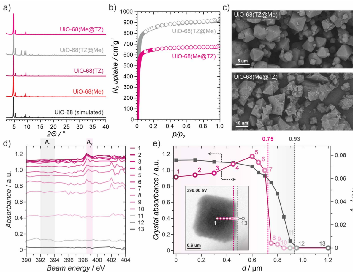
Fig. 3 (a) PXRD patterns of the phase-pure MOFs: UiO-68(TZ), UiO-68(Me), and derived core-shell materials: UiO-68(TZ@Me), UiO-68(Me@TZ), compared to UiO-68 (simulated). (b) N_2 sorption isotherms (at 77 K) of the core-shell materials, closed symbols (adsorption), open symbols (desorption). (c) SEM images of the core-shell materials. (d) X-ray absorption spectra of UiO-68(TZ@Me) collected along the axis from crystal center (points 1–13). Areas A_1 and A_2 marked for the calculation of A_N parameter, for nitrogen abundance estimation. For details see ESI, Section S12† (e) X-ray absorbance at 390 eV for the UiO-68(TZ@Me) crystal probed at 13 points shown in the inset, together with the calculated A_N . The limiting values of both the absorbance at 390 eV and A_N determine the crystal surface boundary (grey dashed line) and the limit of the presence of nitrogen in the crystal (pink dashed line).
