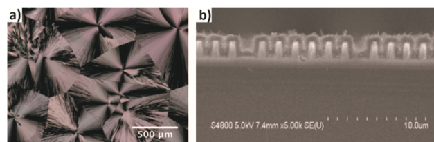
Fig. 7 (a) Optical micrograph image of a film crystallized in moist air. (b) Cross-sectional FESEM image of a MOF-5 film deposited on a silicon substrate with trenches. Reproduced from ref. 58, copyright (2013), with permission from Elsevier.
