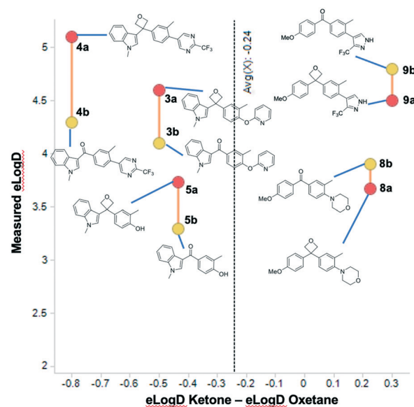
Fig. 4 log D shift of selected ketone and oxetane compounds indicating the difference between oxetane (red circles) and ketone (yellow circles).
