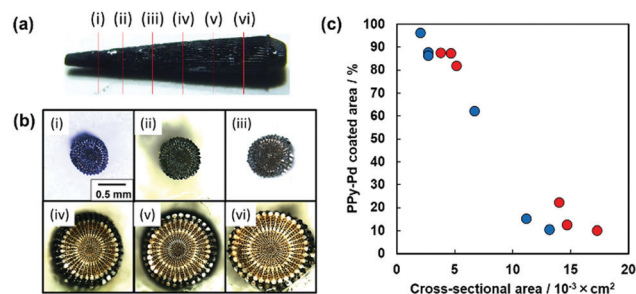
Fig. 3 (a) Optical photograph and (b) cross-sectional optical micrographs of the biomineral after chemical oxidative polymerization of pyrrole with \text{PdCl}_2 oxidant. (c) Relationship between cross-sectional area and PPy-Pd nanocomposite coated area.
