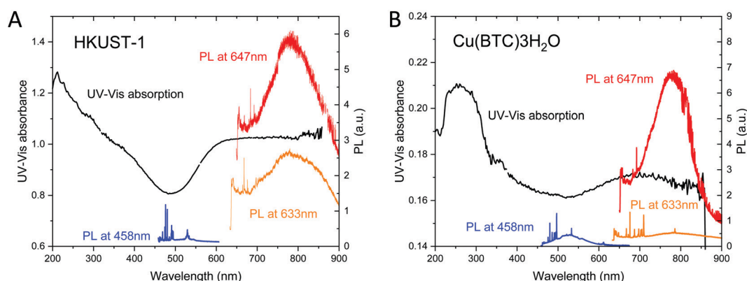
Fig. 6 (A) UV-Vis absorption spectrum of HKUST-1 (black curve). (B) UV-Vis absorption spectrum of \text{Cu}(\text{BTC})\cdot 3\text{H}_2\text{O} (black curve). Their photoluminescence (PL) spectra measured at \lambda = 458, 633 , and 647 nm are also plotted in blue, orange and red, respectively.
