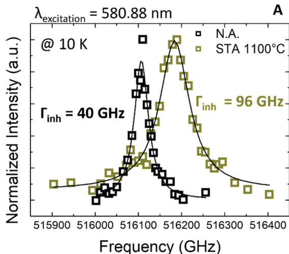
Fig. 4 Inhomogeneous linewidth at 10 K for the as-grown single \text{Eu}:\text{Y}_2\text{O}_3 layer on \text{Si}(111) (N.A.) and after STA annealing at 1100\text{ }^\circ\text{C} for 2 h in air. Solid lines are Lorentzian fits to the experimental data, from which the full width at half maximum (FWHM) are extracted.
