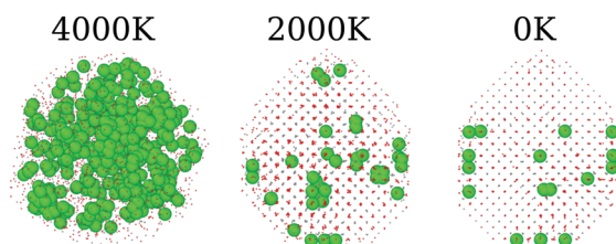
Fig. 8 Vacancy (represented as green spheres) distribution on \text{CeO}_2 pure systems at three different temperatures. The Ce and O atoms are represented by gray and red dots, respectively, for ease of visualization of the vacancy positions.
