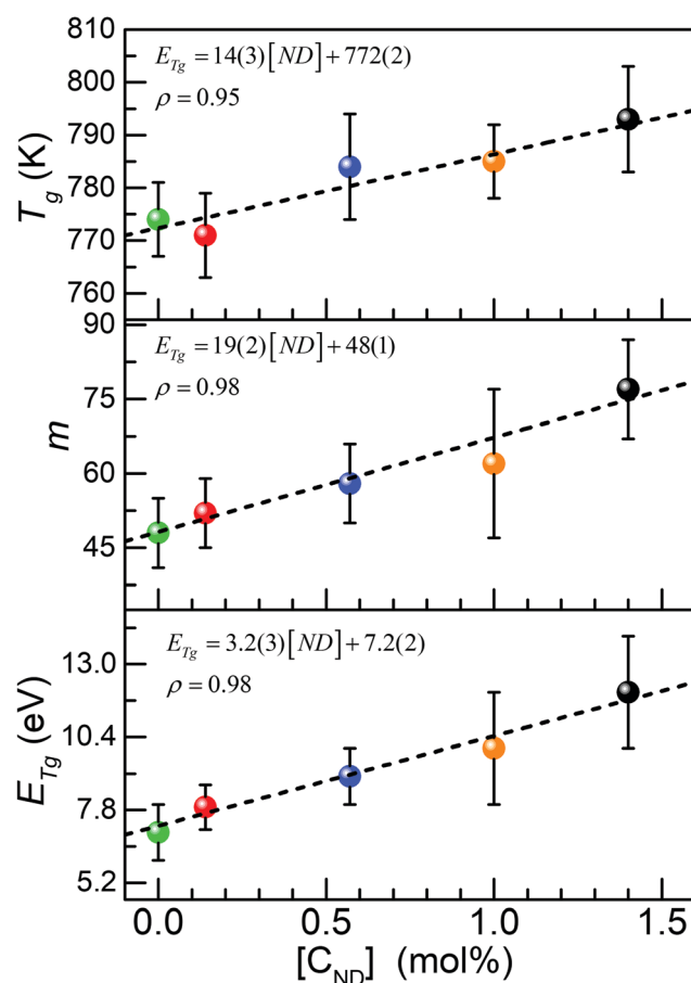
Fig. 8 Glass transition temperature, T_g , at 10^\circ\text{C min}^{-1} (top), liquid fragility, m , (middle) and the glass transition activation energy, E_{Tg} (bottom) as a function of the molar C_{ND} concentration in the melts. The linear regression and the Pearson's coefficients \rho are listed. The data points at 0 mol% stand for the Eu reference glass.
