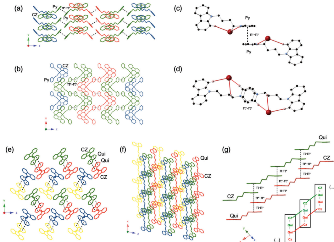
Fig. 1 Different crystal views of the intermolecular packing of Py-Br (a and b) and Qui-Br (e and f). (c and d) Molecular \pi^+ \cdots \pi^+ and Br-H interactions in Py-Br . (g) Molecular \pi-\pi^+ and \pi^+ \cdots \pi^+ interactions in Qui-Br .
