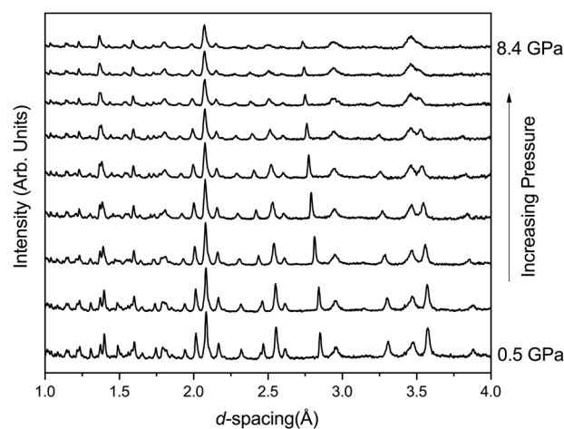
Fig. 3 Neutron diffraction patterns of FePO 4 -II with increasing pressure.
