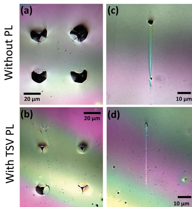
Fig. 5 Optical microscopy photographs of the surface of Tamm plasmon devices with and without PL. Array of 4 indentations up to 1000 nm depth in 4\times(\text{SC}/\text{TB})/\text{Au} (a) and 4\times(\text{SC}/\text{TB})/\text{Au}/\text{TSV} (b); scratches in the same Tamm plasmon devices, without (c) and with (d) TSV PL.
