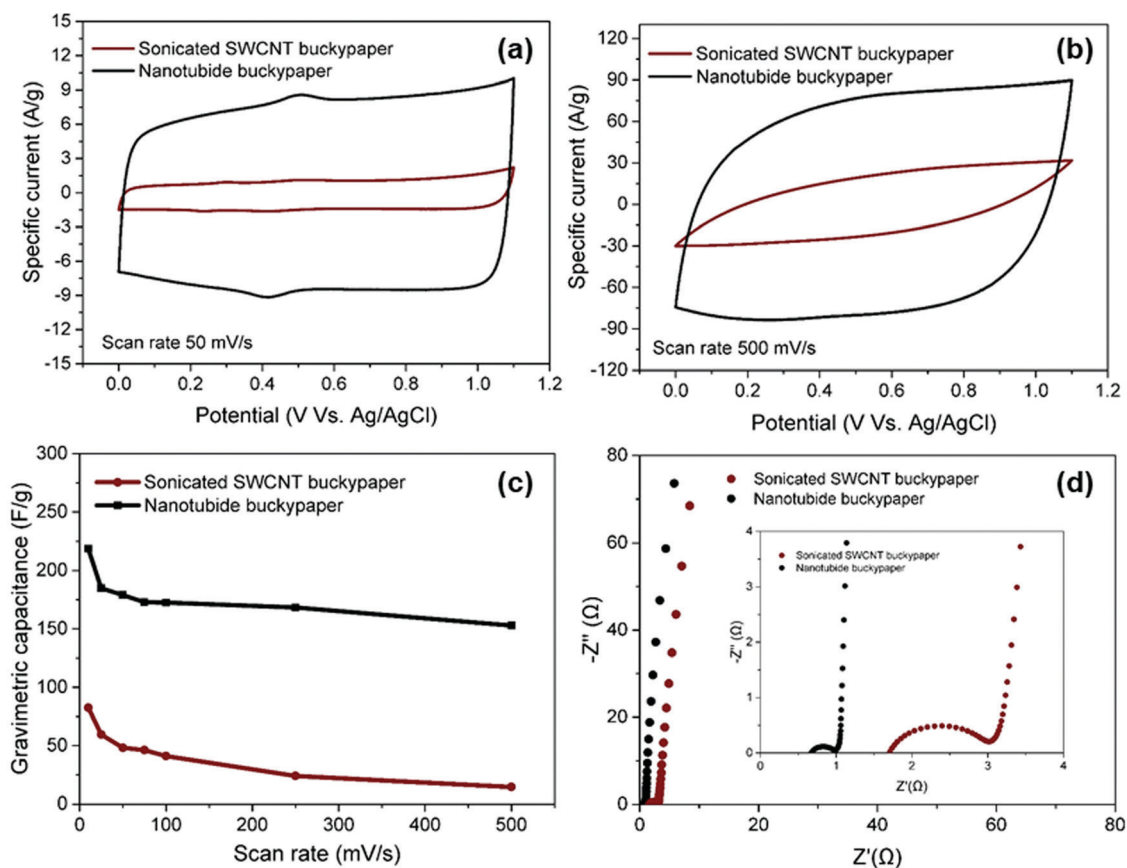
Fig. 3 Half-cell electrochemical performance, in 1 \text{ M H}_2\text{SO}_4 , comparing optimised nanotubide buckypaper to a conventionally processed control: (a) CV curves at 50 \text{ mV s}^{-1} , (b) CV curves at 500 \text{ mV s}^{-1} , (c) gravimetric capacitance as a function of scan rate normalised by mass of active electrode and (d) Nyquist plots.
