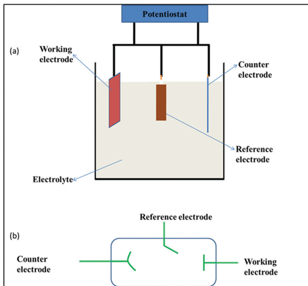
Fig. 17 Schematics presenting the cell connections of the three-electrode system.
