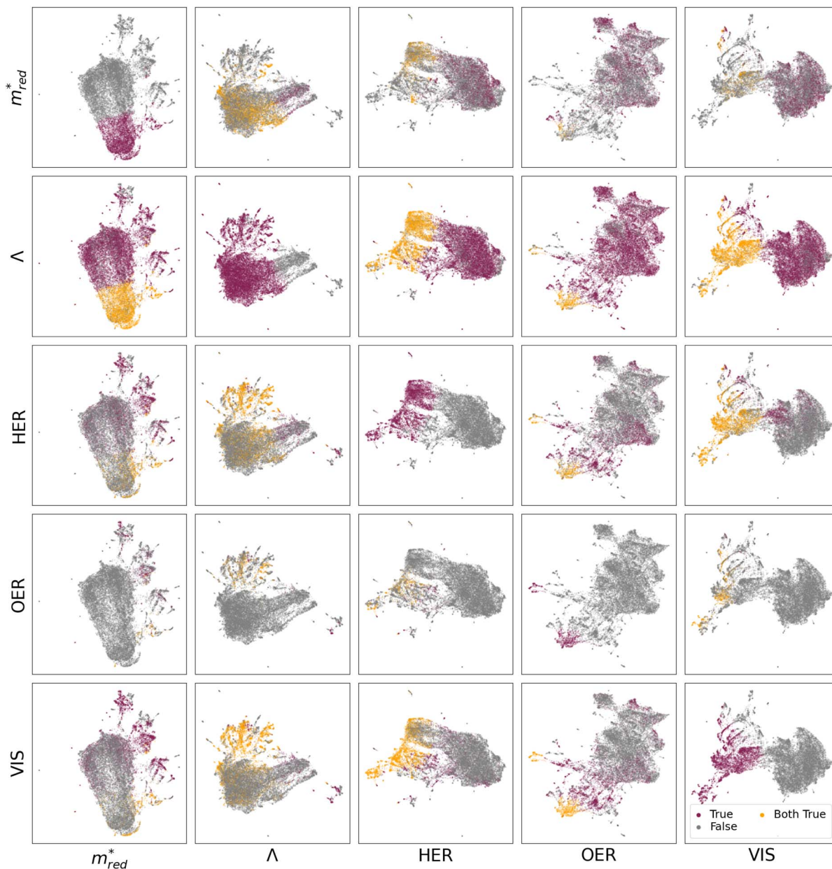
Fig. 3 The five descriptors, charge transport ( m_{\text{red}}^* ), charge separation ( \Delta ), visible light absorption (VIS), and alignment to the photoredox reactions (HER and OER), shown in chemical design space. These figures show a UMAP projection of the 768-dimensional vector characterizing the similarity of MOF fine-tuned on one of the descriptors. All figures in a column are fine-tuned on the same descriptor X . Each row represents a different descriptor Y ; a MOF is represented with a grey dot if the criteria of descriptor Y are not met and a purple dot if the criteria are met. A MOF is represented with an orange dot if the MOF meets both criteria Y and X . Hence, the diagonal ( X, X ) has only grey and purple dots, and the number of orange dots in figures ( Y, X ) and ( X, Y ) is by definition equal.
