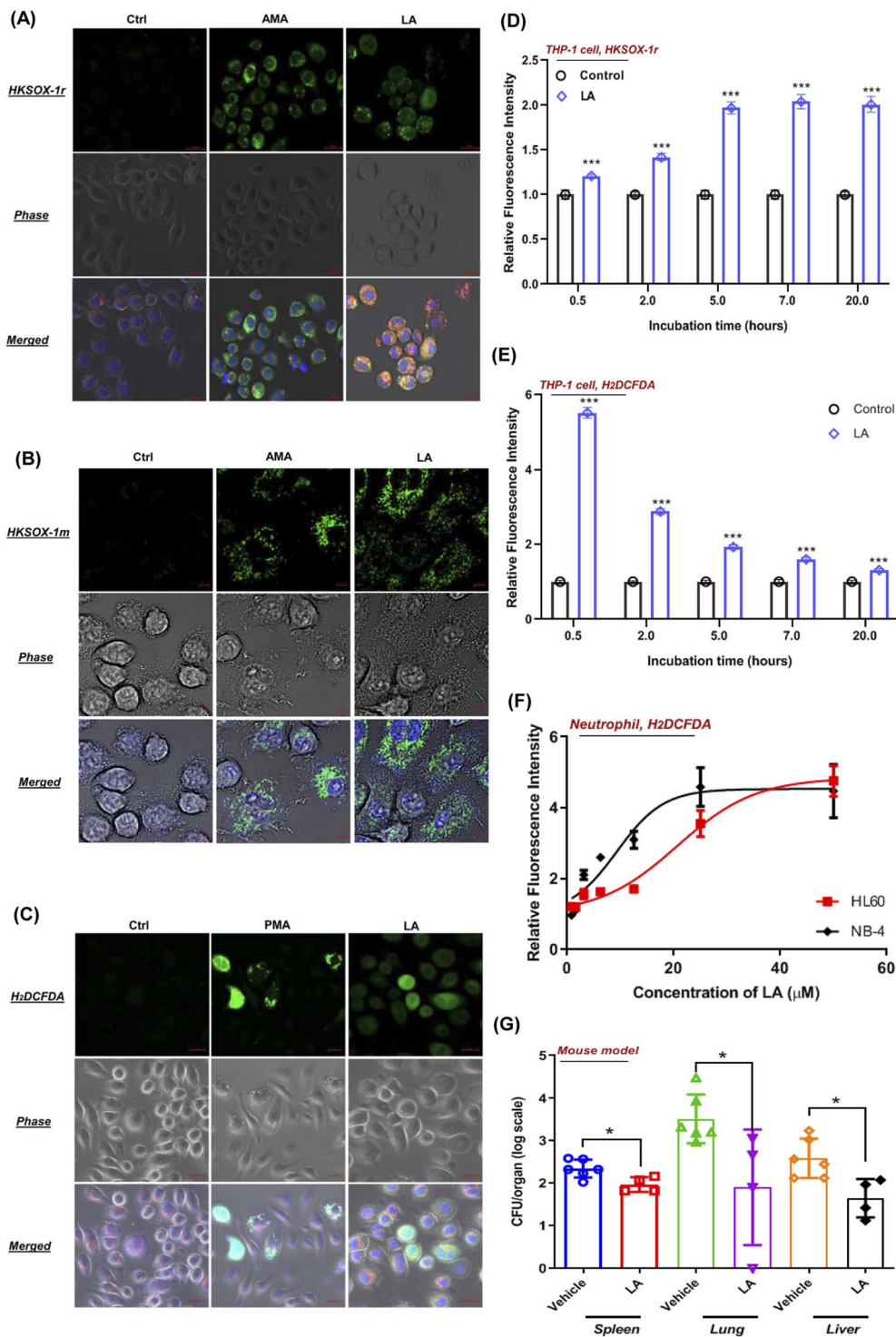
Fig. 7 LA induced ROS production in living phagocytes and neutrophils. (A) Representative images of a J774A.1 cell stimulated with AMA (5 \mu M) or LA (25 \mu M), and co-cubated with HKSOX-1r (2 \mu M) for 30 min before confocal imaging. (B) Representative images of a J774A.1 cell stimulated with AMA (5 \mu M) or LA (25 \mu M), and co-cubated with HKSOX-1m (10 \mu M) for 30 min before confocal imaging. (C) Representative images of a J774A.1 cell stimulated with PMA (100 nM) or LA (25 \mu M) and co-cubated with H 2 DCFDA (6 \mu M) for 30 min before confocal imaging. Cells were costained with mitochondrial dye MitoTracker Red (50 nM), nuclear DNA dye Hoechst 33342 (150 ng mL -1 ), and probes for 30 min before confocal imaging. The compound was kept incubated with cells during the image capture. Merged: all fluorescence images merged. Scale bar = 20 \mu m. (D and E) Fluorescence intensities of superoxide (D) and ROS (H 2 DCFDA probe) (E) upon LA (25 \mu M) induction at indicated incubation times in THP-1 cells. (F) Fluorescence intensities of ROS (H 2 DCFDA probe) upon LA induction at different concentrations in HL-60 and NB-4 differentiated neutrophils. (G) Mice organs such as lungs, livers and spleens were harvested, and bacterial load was analyzed by viable count respectively. Data represent mean \pm SD. One-way ANOVA was used when compared with the vehicle group. For all statistical analysis above, * p < 0.05, ** p < 0.01 and *** p < 0.001.
