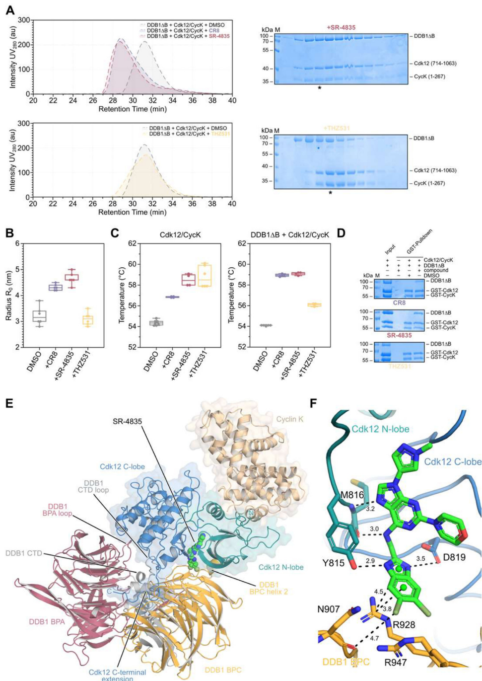
Fig. 3 SR-4835 induces ternary complex formation between Cdk12/CycK and DDB1. (A) Analytical size exclusion chromatography of purified, recombinant DDB1 \Delta B and Cdk12/CycK proteins (20 \mu M) in presence of either 2% DMSO or 60 \mu M small molecular compounds CR8, SR-4835, or THZ531. Peak fractions were analyzed by SDS-PAGE, giving rise to a SR-4835-induced ternary complex between Cdk12/CycK and DDB1 \Delta B, compared to THZ531-treated negative control. Samples highlighted with asterisk were subsequently analyzed by DLS. (B) Dynamic light scattering analysis of peak middle fractions of previously conducted analytical size exclusion chromatography runs (in A). Hydrodynamic radii of CR8, and SR-4835-treated samples are significantly increased compared to negative controls, indicating ternary complex formation. Box-plots display the median of 6 data points per sample, each equivalent to the average of 20 DLS measurements. (C) Thermal stability analysis using the nanoDSF method of compound-treated Cdk12/CycK (left panel) and a mixture of compound-treated DDB1 \Delta B and Cdk12/CycK (right panel). All compounds including THZ531 stabilized Cdk12/CycK kinase. Degradator compounds elevated their stabilizing effects in presence of DDB1 \Delta B, indicating ternary complex formation, while THZ531 only stabilized Cdk12/CycK. (D) pull-down assays using GST-tagged variants of Cdk12 and CycK, identifying drug-induced recruitment of DDB1 in CR8- and SR-4835-treated samples. (E) Cartoon representation of the ternary complex structure of DDB1-SR-4835-Cdk12/CycK at a resolution of 3.9 Å (PDB: 9FMR). (F) Close-up of the SR-4835-linked interface between Cdk12 (C-lobe, blue; N-lobe, turquoise) and the DDB1 \Delta B BPC domain (bright orange), identifying key stacking interactions between the benzimidazole moiety of SR4835 with DDB1 residue R928. Key residues forming the interface are highlighted.
