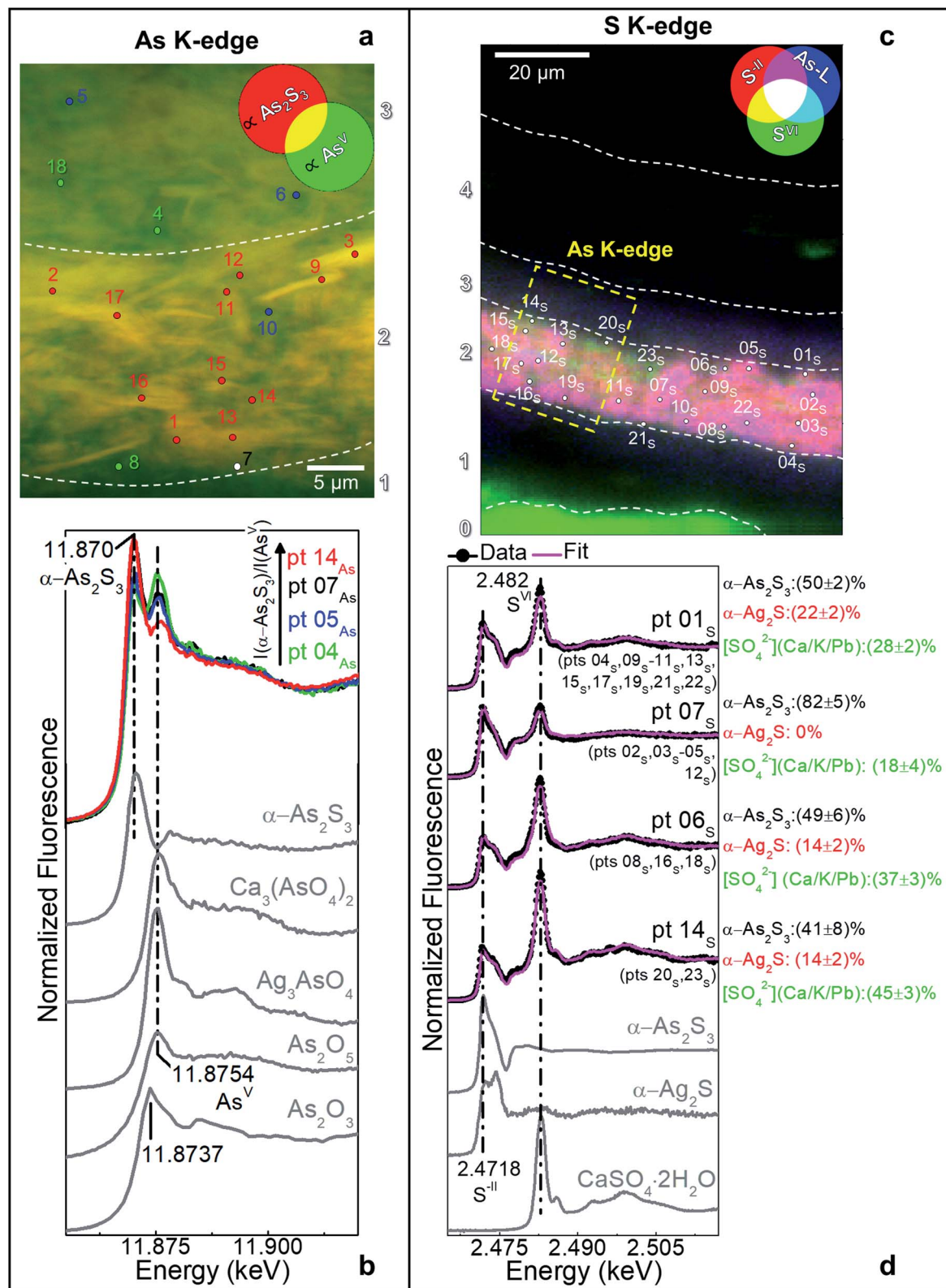
Fig. 2 (a) Composite SR- \mu -XRF images of As III ( \alpha\text{-As}_2\text{S}_3 ) (red) and As V (green) [map size ( v \times h ): 30.7 \times 38.1 \mu\text{m}^2 ; step size ( v \times h ): 0.1 \times 0.1 \mu\text{m}^2 ; exp. time: 100 ms per pixel; energy (As III ) = 11.870 keV, energy (As V ) = 11.8754 keV] and (b) selection of the As K-edge \mu -XANES spectra acquired from the spots shown in (a) compared to those of a set of As-reference compounds. Different colors refer to spectra characterized by similar features and showing a variable ratio between the intensity of the white lines of \alpha\text{-As}_2\text{S}_3 and As V -compounds. (c) RGB SR- \mu -XRF images of S II /S VI /As-L [map size ( v \times h ): 99.5 \times 74.2 \mu\text{m}^2 ; step size ( v \times h ): 0.5 \times 0.7 \mu\text{m}^2 ; exp. time: 100 ms per pixel; energy (S II ) = 2.4718 keV, energy (S VI ) = 2.482 keV] and (d) selection of the S K-edge \mu -XANES spectra (black) recorded from the spots shown in (c) with LCF results (magenta) of different S-reference compounds. In grey, spectra of selected S-reference compounds. Numbers in brackets refer to the spectral profiles showing similar features to those reported.
