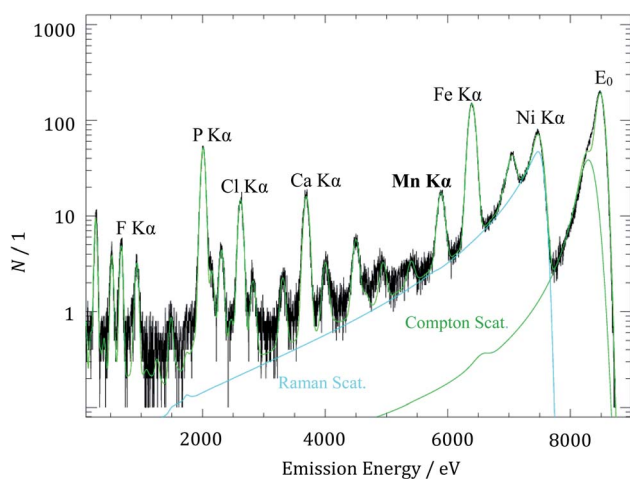
Fig. 3 X-ray fluorescence spectrum of the aged anode for the determination of manganese mass deposition with an excitation energy E_0 of 8500 eV.
