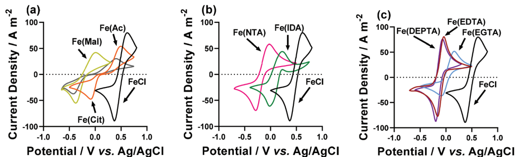
Fig. 4 Cyclic voltammograms of (a) Fe(Ac), Fe(Mal) and Fe(Cit), (b) Fe(IDA) and Fe(NTA) and (c) Fe(EDTA), Fe(EGTA) and Fe(DEPTA) redox couples; all are compared to the parent \text{FeCl}_{2/3} species ( i.e. 50 mM \text{FeCl}_2 and 50 mM \text{FeCl}_3 , in the absence of any ligand). All voltammograms were recorded at an Au working electrode, at a scan rate of 50 \text{ mV s}^{-1} and ambient temperature.
