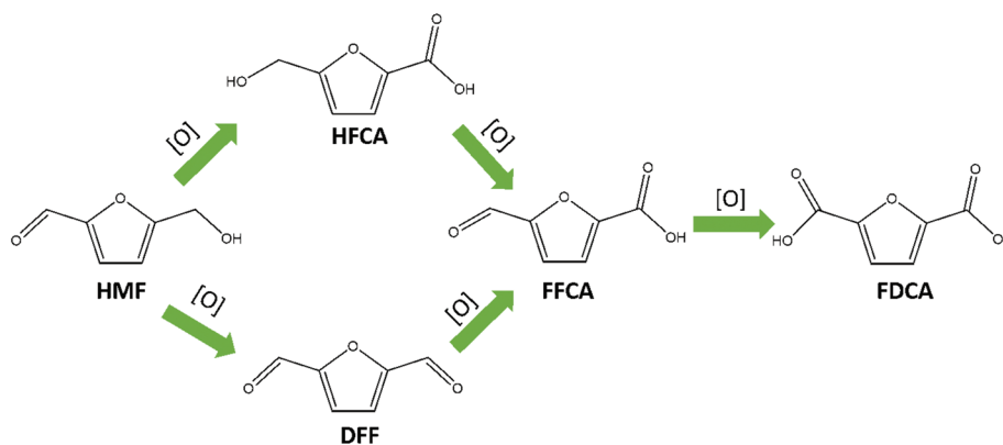
Scheme 1 Electrochemical HMF oxidation reaction pathways. HMF is converted to DFF (diformyl furan) or HFCAs (hydroxymethyl furan carboxylic acid), which are then further oxidized to FFCA (formyl furan carboxylic acid) and finally to FDCA (2,5-furandicarboxylic acid).
