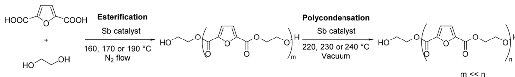
Scheme 1 Polymerization of 2,5-furandicarboxylic acid with ethylene glycol. The first step, the esterification, affords oligomers. The second step, the polycondensation, yields poly(ethylene furanate).
