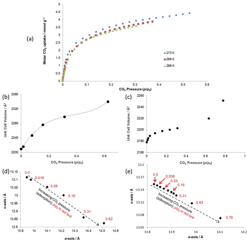
Fig. 6 (a) Gravimetric \text{CO}_2 adsorption isotherms at 273, 288 and 298 K for SHF-81 (activated from SHF-81-DMF ). Unit cell volume of SHF-81 as a function of \text{CO}_2 pressure during (b) in situ SCXRD study at 298 K and (c) in situ PXRD study at 298 K. Lattice parameters for SHF-81 as a function of increasing \text{CO}_2 pressure during (d) in situ SCXRD study at 298 K and (e) in situ PXRD study at 298 K. The dotted line in (b) is a guide to the eye, and illustrates the likely inflexion point slightly below p/p_0 0.6. The arrows in (d) and (e) represent the direction of change for increasing \text{CO}_2 pressure (adsorption).
