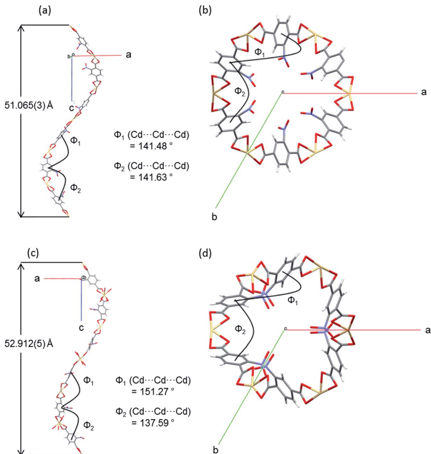
Fig. 4 A single turn of a helix viewed perpendicular and parallel to the c -axis, along which the helices and accompanying pores propagate, shown with dimensions for alternating Cd⋯Cd⋯Cd angles ( \varphi_1 , \varphi_2 ) and the helix pitch, for (a) and (b) SHF-81-DMF; (c) and (d) SHF-81. Single-crystal structures determined at 100 K.
