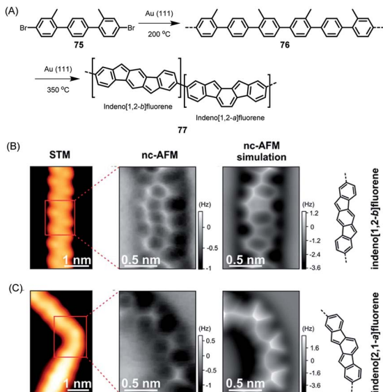
Fig. 10 (A) On-surface synthesis of indenofluorene-based polymer 77 . (B and C) STM images, constant-height frequency-shift nc-AFM images, simulated nc-AFM images and chemical structures of the straight and bent segments of 77 . 180 Copyright 2017. Adapted with permission from the American Chemical Society.
