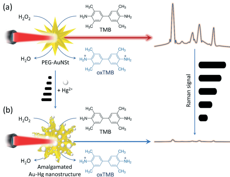
Scheme 1 Working principle of the SERS-sensing approach using catalytic AuNst for the detection of \text{Hg}^{2+} ions. (a) In the presence of AuNst-PEG, 1.25 mM TMB and 6% \text{H}_2\text{O}_2 , TMB is catalysed into a highly Raman active product (oxTMB) that allows a strong SERS intensity to be measured using the PEG-AuNst. (b) The catalytic activity of AuNst-PEG remains in the presence of \text{Hg}^{2+} ions. However, decreased SERS intensity is observed when the morphology of the AuNst-PEG is altered as a result of Au-Hg amalgamation.
