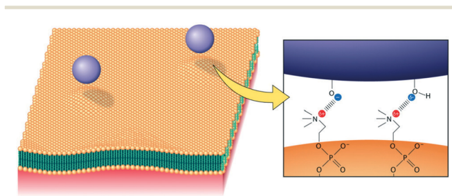
Fig. 5 Schematic representation of the interaction mechanism of silica NPs and cellular membranes at physiological pH: membrane phospholipids interacts either with deprotonated geminal and vicinal silanols through ionic interactions, or with isolated silanols through hydrogen bonds. Reproduced from ref. 87 with permission from Elsevier, copyright 2016.
