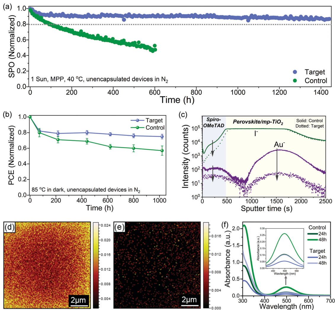
Fig. 4 Stability measurements and degradation mechanism. (a) Maximum power point tracking measured with the unencapsulated device white LED light ( 100 \text{ mW cm}^{-2} in \text{N}_2 , 40 \text{ }^\circ\text{C} ). The initial stabilized power output (SPO) for control and target was 19.7% and 20.9%, respectively. (b) Thermal stability of devices at a fixed temperature of 85 \text{ }^\circ\text{C} in a nitrogen atmosphere. Statistical data of four devices for each control and target. The data points (color-filled dots) were collected by measuring the J - V curves of the devices at different time intervals. The initial PCE for best control and target was 20.6% and 21.5%, respectively. (c) TOF-SIMS depth profile for the aged devices. (d) and (e) TOF-SIMS 2D images of \text{I}^- ion signal on the spiro-OMeTAD surface ( 10 \mu\text{m} \times 10 \mu\text{m} ) for (d) control and (e) target devices. The color scale for each image is normalized intensity per pixel. For TOF-SIMS the samples were aged after 350 hours of light-soaking at the maximum power point at 40 \text{ }^\circ\text{C} , and after aging, gold was exfoliated by the scotch tape. (f) UV-vis absorbance spectra recorded for the toluene solution taken from the control and target vials at 24 and 48 h. The band at 500 nm corresponds to \text{I}_2 and is zoomed in the inset.
