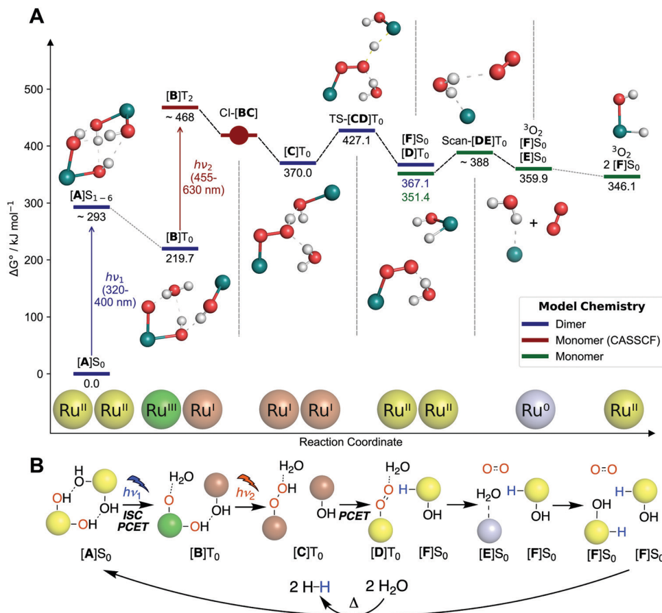
Fig. 5 (A) DFT computed free energy profile. Energies of excited species ([A]S 1-6 and [B]T 2 ) are only approximate. Franck–Condon geometry is shown for [A]S 1-6 . Abbreviations: “CI” conical intersections, “TS” transition state, “Scan” relaxed potential energy surface scan. (B) Schematic representation of mechanism shown in (A). Colored spheres indicate ruthenium centers with corresponding formal oxidation states (Ru 0 = grey, Ru I = brown, Ru II = yellow, Ru III = green). Abbreviations: “ISC” intersystem crossing, “PCET” proton-coupled electron transfer. Shown oxidation states are only formal to visualize electron flow. Structures are shown without other ligands for clarity.
