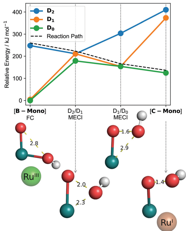
Fig. 6 CASSCF computed reaction from [B-Mono] to [C-Mono] including minimum energy conical intersections (MECI). Bond distances are in Ångström. Calculations in the gas phase, for solution phase results see ESI,† Fig. S11.3-1. "FC" refers to Franck-Condon geometry. Shown oxidation states are only formal to visualize electron flow. Structures are shown without other ligands for clarity.
