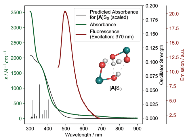
Fig. 2 Experimental (green) and theoretical (black) absorbance of 1 (theoretical model [\text{A}]S_0 , see below) as well experimental fluorescence (red). Individual theoretical transitions are shown as vertical lines. Inset shows structure of [\text{A}]S_0 with other ligands omitted for clarity.
