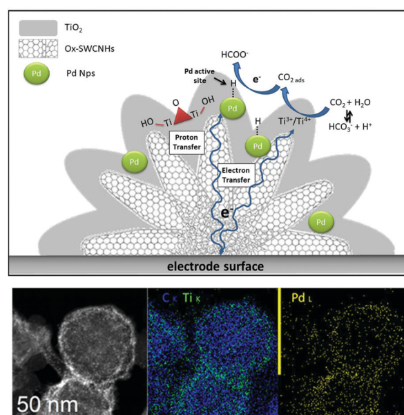
Fig. 6 Top: Graphical sketch of the PdNP/ \text{TiO}_2\text{@CNH} nano hybrid and of the interfacial synergy towards the reversible \text{HCOOH} formation; bottom: HAAFD (black and white) and EDX elemental mapping of C, Ti and Pd confirming the co-location of the three elements.
