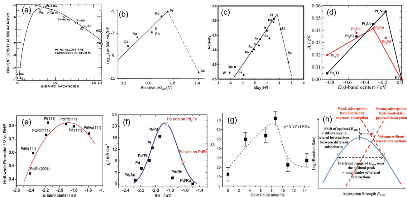
Fig. 5 Volcano plots of ORR activity vs. various elements. (a) \text{O}_2 reduction in 85% orthophosphoric acid: the plot of current density at q = -460 mV at 25^\circ\text{C} against the d-orbital vacancy value of the electrode metal. Reproduced with permission. 63 Copyright 1971, Taylor & Francis. (b) Volcano plots of current density i in the ORR vs. relative \Delta G_{\text{ads}} . Reproduced with permission. 37 Copyright 1983, Springer. (c) Trends in ORR activity plotted as a function of the oxygen binding energy. Reproduced with permission. 61 Copyright 2004, American Chemical Society. (d) The volcano plot of ORR activity vs. the experimentally measured d-band center. Reproduced with permission. 64 Copyright 2006, Wiley-VCH. (e) The volcano plot of the half-wave potential of Pd-based alloys as a function of the calculated Pd d-band center (relative to the Fermi level). Reproduced with permission. 65 Copyright 2006, American Chemical Society. (f) Volcano plots of the ORR activity (expressed as the kinetic current density) vs. the calculated oxygen-binding energy. Reproduced with permission. 66 Copyright 2007, American Chemical Society. (g) The volcano-type relationship between the surface-specific activity (SA) of Pd–Co alloys and the degree of alloying. Reproduced with permission. 57 Copyright 2007, Wiley-VCH. (h) The relationship between the catalytic activity and the adsorption strength for certain surface reactions. Reproduced with permission. 68 Copyright 2012, Elsevier.
