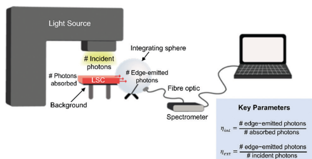
Fig. 2 Experimental configurations used for the characterization of LSCs. (a) The optical characterisation of LSCs is carried out by irradiating the top surface of the LSC with a calibrated light source of known intensity and measuring the edge-emitted light during exposure by means of an integrating sphere coupled to a suitable detector. The key parameters extracted are the internal photon efficiency \eta_{\text{int}} and the external photon efficiency \eta_{\text{ext}} , as defined in the light-blue box and discussed in the main text. (b) The device characterization of LSCs is performed by recording the J – V curve of edge-mounted solar cells of known spectral response under controlled illumination of the LSC top surface (typically, AM 1.5G simulated solar light). The key parameter extracted is the device efficiency \eta_{\text{dev}} , as defined in the light-blue box and discussed in the main text.
