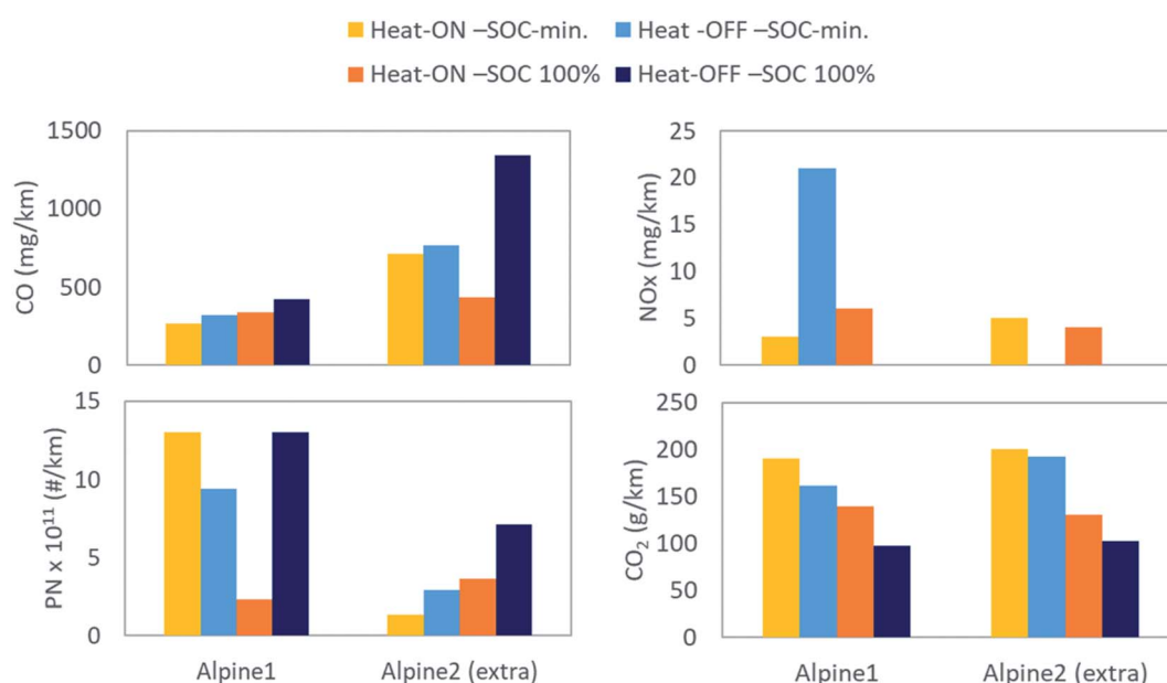
Fig. 7 Emission factors of PHEV for \text{NOx} , CO, PN, and \text{CO}_2 , corresponding to the complete on-road tests during the Alpine1 and Alpine2 (extra) tests. All tests were performed with the PHEV at depleted battery (SOC-min) and 100% battery SOC and with the air conditioning heating system enabled (Heat-ON) and disabled (Heat-OFF). Coolant temperature ranged between 4^{\circ}\text{C} and 8^{\circ}\text{C} . Emissions factors for the test Alpine1 – Heat-OFF – SOC-min (light blue bars) were calculated by correcting a shift on the exhaust flow rate and multiplying it by a 3.7 factor. Therefore, the values should be taken as indicative.
