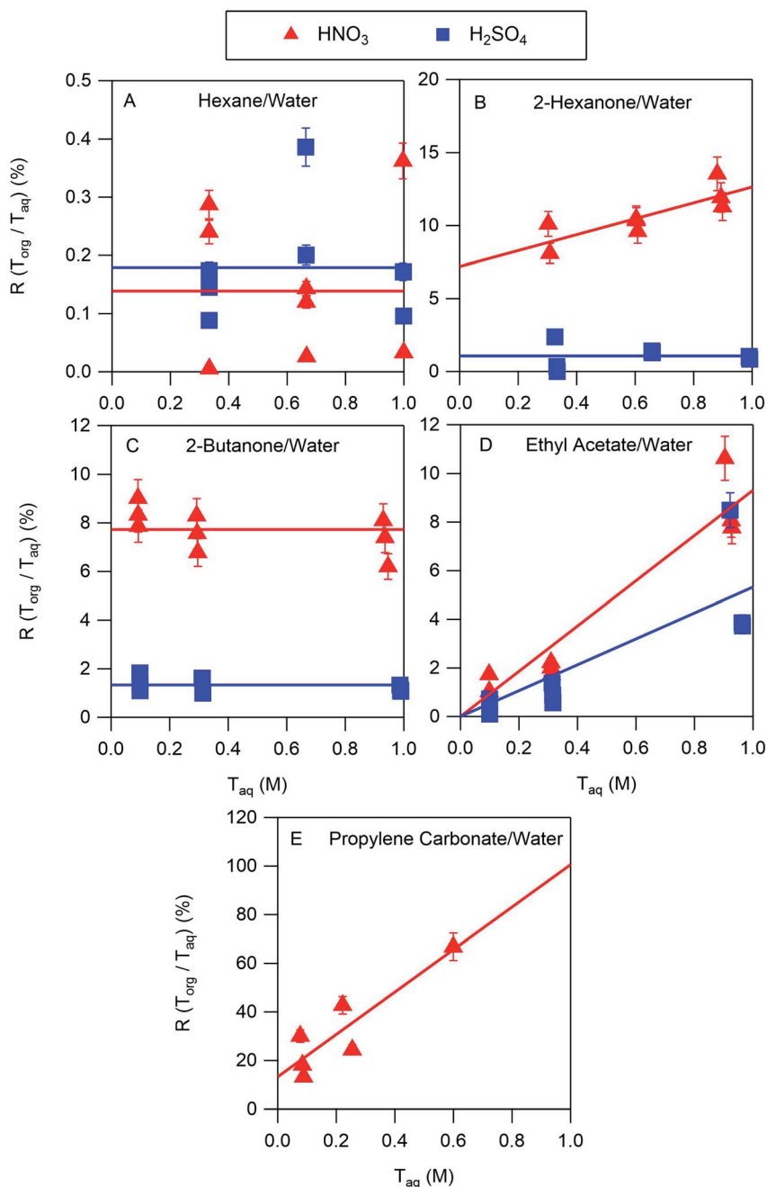
Fig. 2 Ratios of organic-phase acid/aqueous-phase acid, R(T_{org}/T_{aq}) , measured for HNO_3 and H_2SO_4 as a function of the aqueous-phase acid concentration, with (A) hexane, (B) 2-hexanone, (C) 2-butanone, (D) ethyl acetate, and (E) propylene carbonate as the organic phase. Lines are linear least squares fits to the data, with slopes set to zero when the uncertainty exceeds the value and y -intercepts set to zero when values are negative. The error bars correspond to \pm one standard deviation calculated from the expected uncertainties in the mass and volume measurements, and in many cases fall within the symbol.
