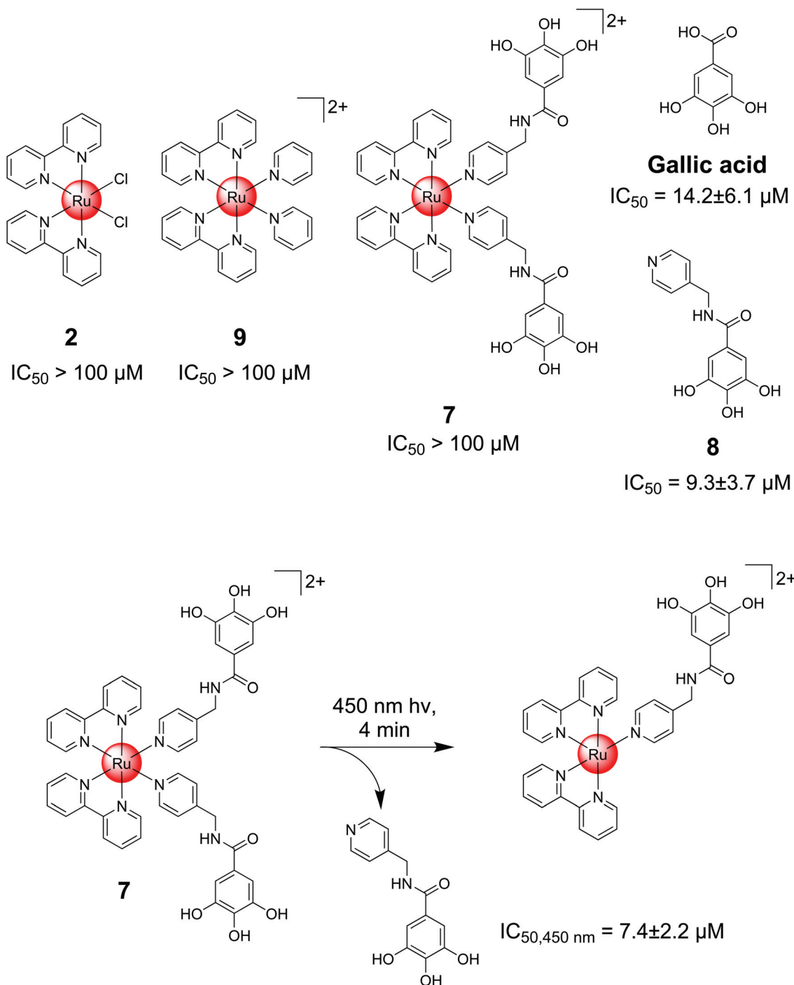
Fig. 4 Structure and inhibition values for compounds 2 , 7 , 8 , 9 , and gallic acid in the dark and for compound 7 upon irradiation at 450 nm.
