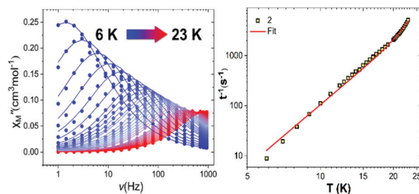
Fig. 3 (Left) Frequency dependence of the out-of-phase, \chi''_M ac susceptibility, in zero dc field, for 2 . The solid lines correspond to the best fit to Debye's law. 46 (Right) Log–Log plot of the relaxation times, \tau^{-1} versus T for 2 (see main text for details).
