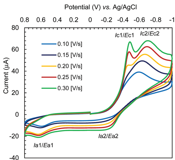
Fig. 10 Cyclic voltammograms for \text{Cu-R-L}^1 ( 0.5 mM); TBAP ( 0.1 M) at varying scan rates 0.10 – 0.30 V \text{s}^{-1} in acetonitrile at 25^\circ\text{C} .
