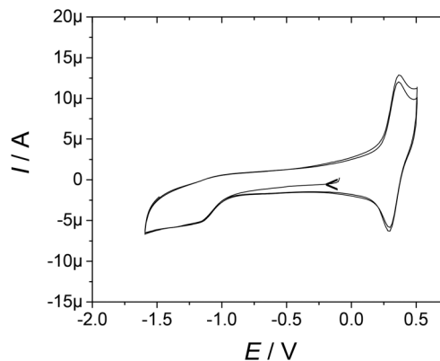
Fig. 2 Cyclic voltammogram curve of [\text{Eu}(\text{L}_2)]^{3+} in 0.5 mM \text{CH}_3\text{CN} solution containing 0.1 M TBAP. Scan rate, 0.1 \text{ V s}^{-1} ; T = 298 K; carbon electrode.
