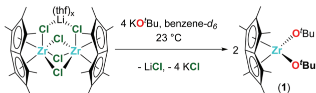
Chart 1 Synthesis of \text{Pn}^*\text{Zr}(\text{O}^t\text{Bu})_2 ( 1 ).
