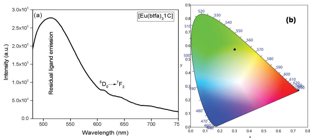
Fig. 5 (a) Emission spectrum in DCM at RT at 464 nm, (b) CIE-1931 chromaticity diagram demonstrating the calculated color coordinate ( x , y ) values for [\text{Eu}(\text{btfa})_3\mathbf{1c}] complex.
